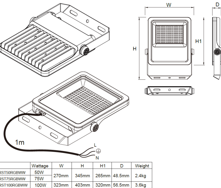
Dimension Diagram
